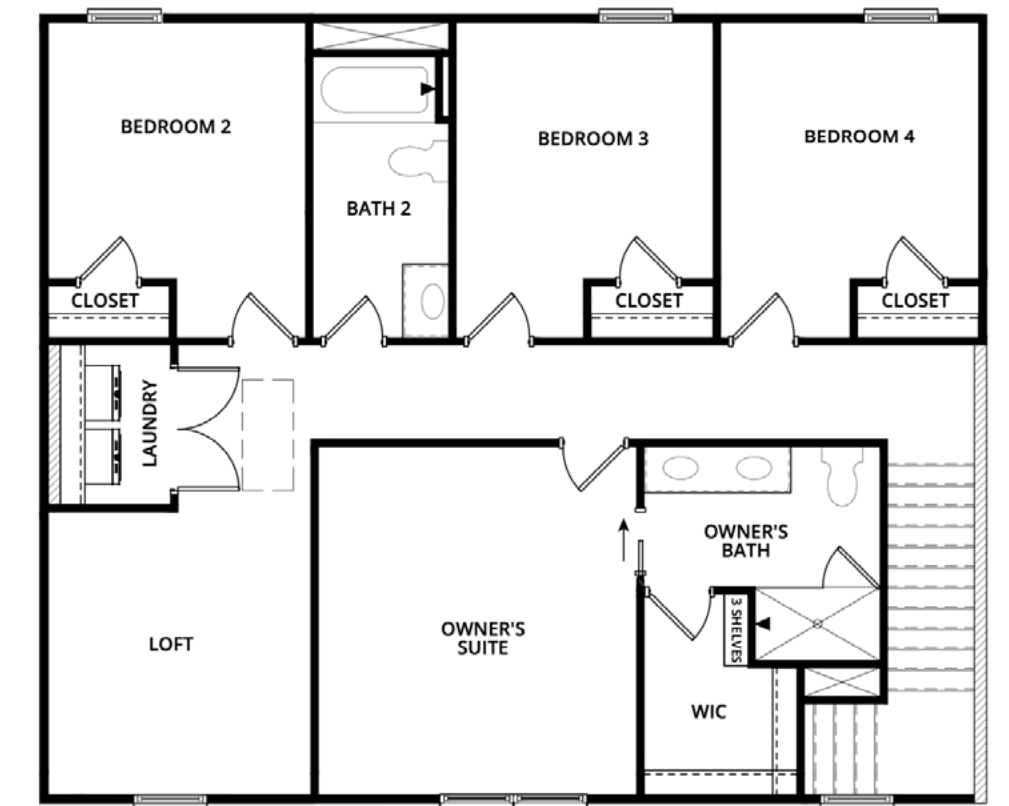
SECOND FLOOR PLAN 30
